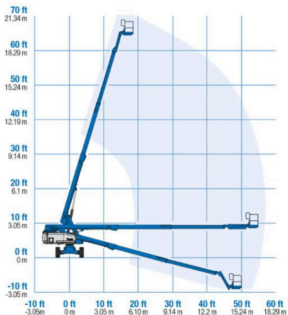
Range Of Motion S-65 (500 lb capacity)
